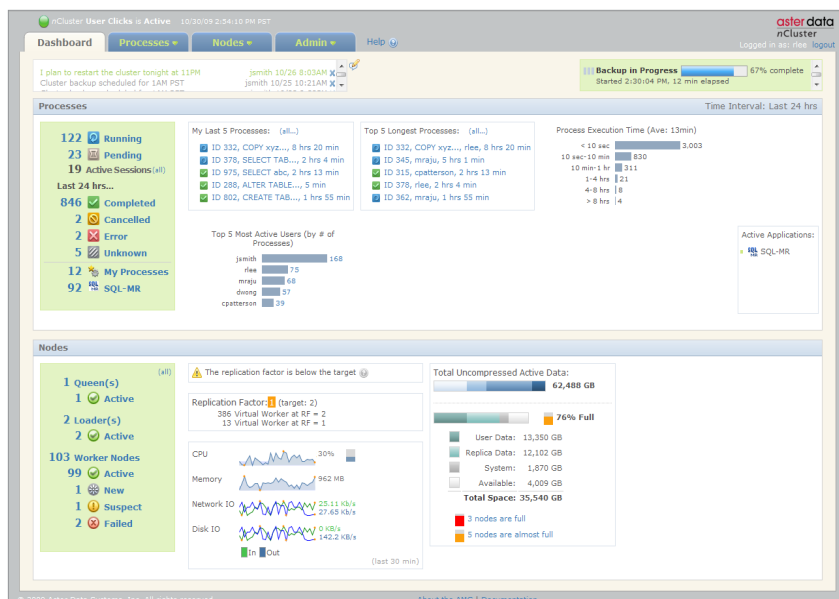
Figure 1: Aster Data Management Console
